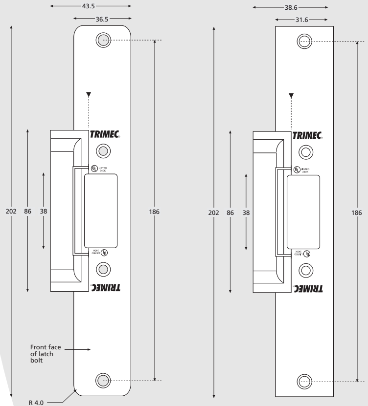
(AS) ANSI Short Faceplate
