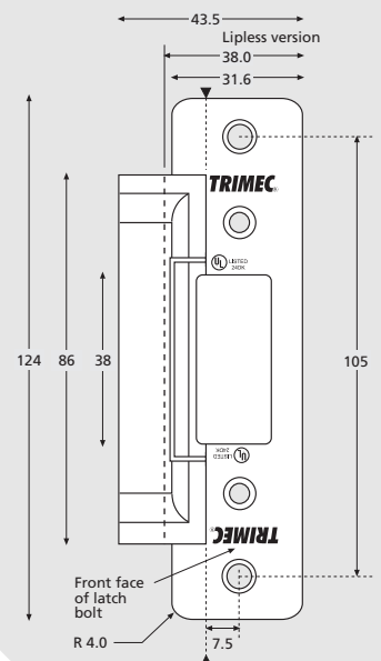
(AS) ANSI Short Faceplate
