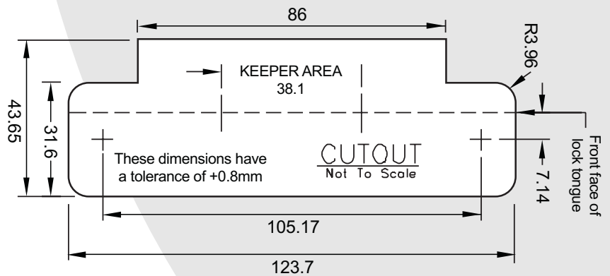
(AS) ANSI Short Faceplate
