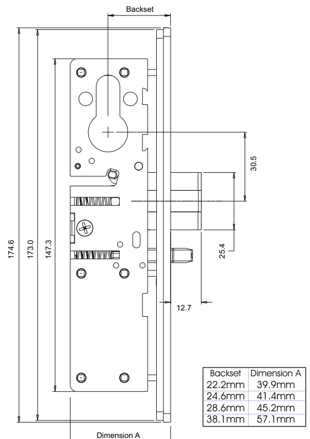
52FP4511 Faceplate
